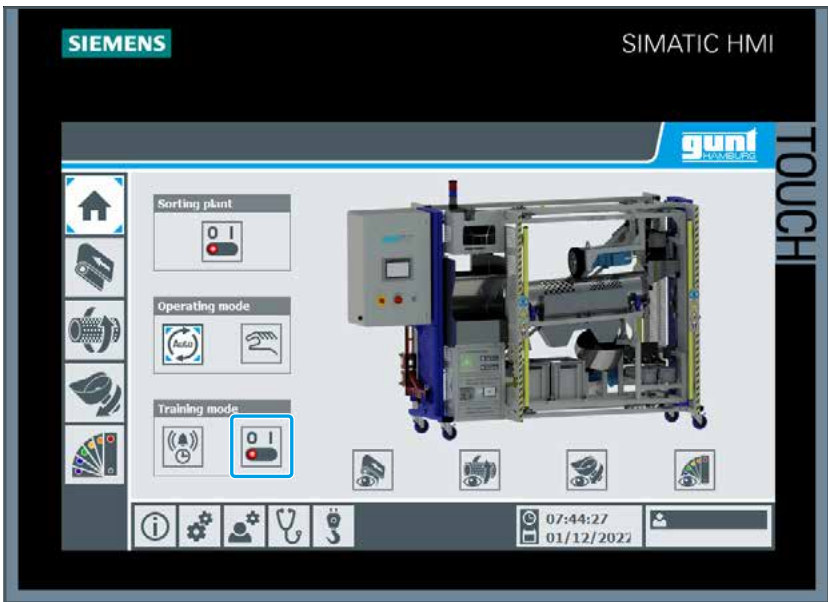
Switch on training mode on the touch screen. Operating hours counter is located in the PLC. The maintenance intervals for the various sub-systems can be simulated , i.e. adjusted.
