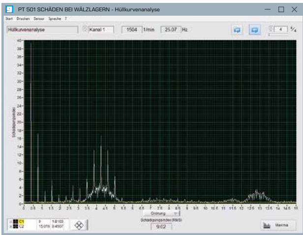
The GUNT software for vibration analysis allows versatile display and analysis options. Software and control unit are included in the scope of delivery.
