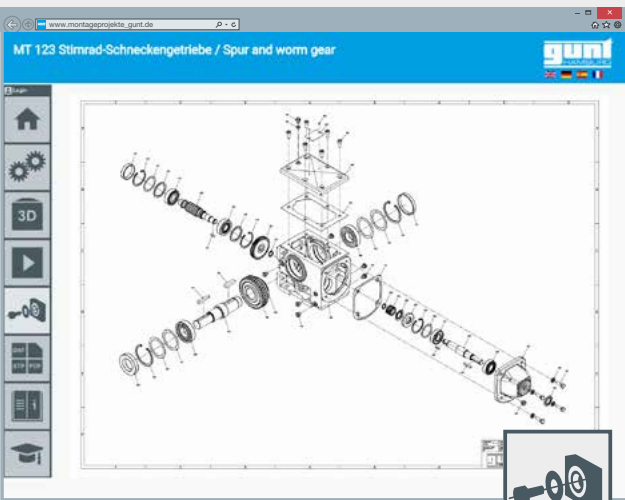
exploded drawings
