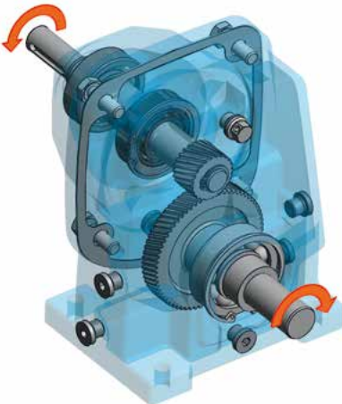
MT 120 Assembly exercise: spur gear
